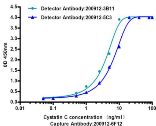
Standard Curve for Human Cystatin C: Capture Antibody Mouse mAb [6F12-C7-D8] to Human Cystatin C at 4µg/ml and Detector Antibody Mouse mAb [200912-5C3:5C3-C7.200912-3B11:3B11-E9]to Human Cystatin C at 0.5µg/ml.
