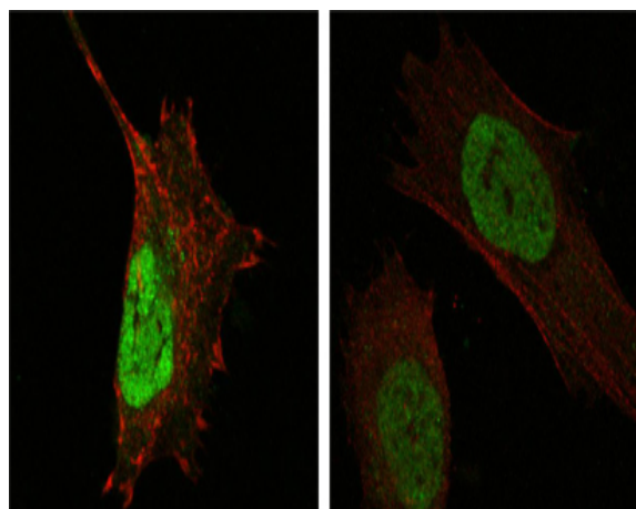
Confocal immunofluorescence analysis of HeLa (left) and L-02 (right) cells using MDMX Monoclonal Antibody (green). Red: Actin filaments have been labeled with DY-554 phalloidin.
