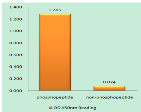
Enzyme-Linked Immunosorbent Assay (Phospho-ELISA) for Immunogen Phosphopeptide (Phospho-left) and Non-Phosphopeptide (Phospho-right), using BCL-XL (Phospho-Thr47) Antibody
