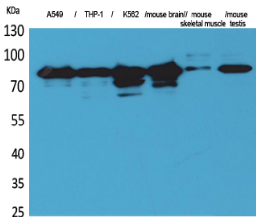
Western Blot analysis of A549, THP-1, K562, mouse brain, mouse skeletal muscle, mouse testis cells using PKC \gamma Polyclonal Antibody. Secondary antibody(catalog#:RS0002) was diluted at 1:20000
