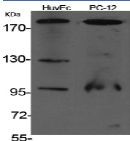
ABCA8 Western Blot analysis of various cells using ABCA8 Polyclonal Antibody
