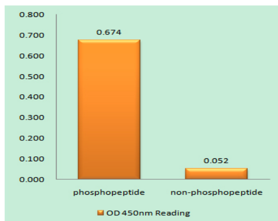
Enzyme-Linked Immunosorbent Assay (Phospho-ELISA) for Immunogen Phosphopeptide (Phospho-left) and Non-Phosphopeptide (Phospho-right), using LKB1 (Phospho-Thr189) Antibody
